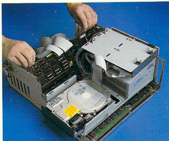
Step 3. Installing the hard-drive controller into the first Amiga slot.
